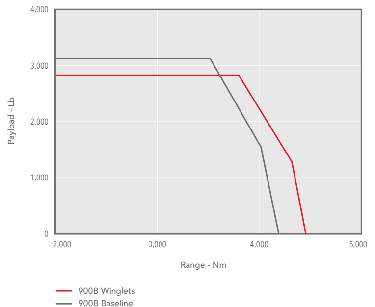
FALCON 900B PAYLOAD RANGE
