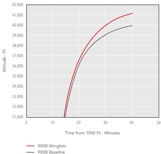
FALCON 900B CLIMB TIME
