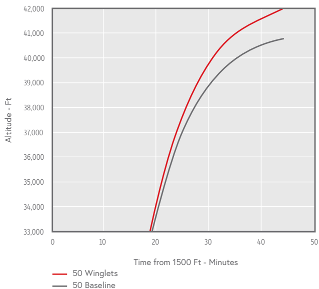
FALCON 50 CLIMB TIME
