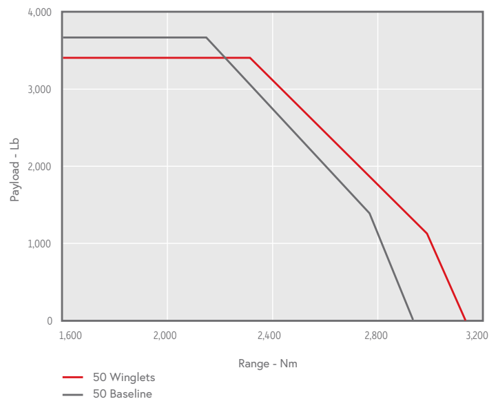
FALCON 50 PAYLOAD RANGE
