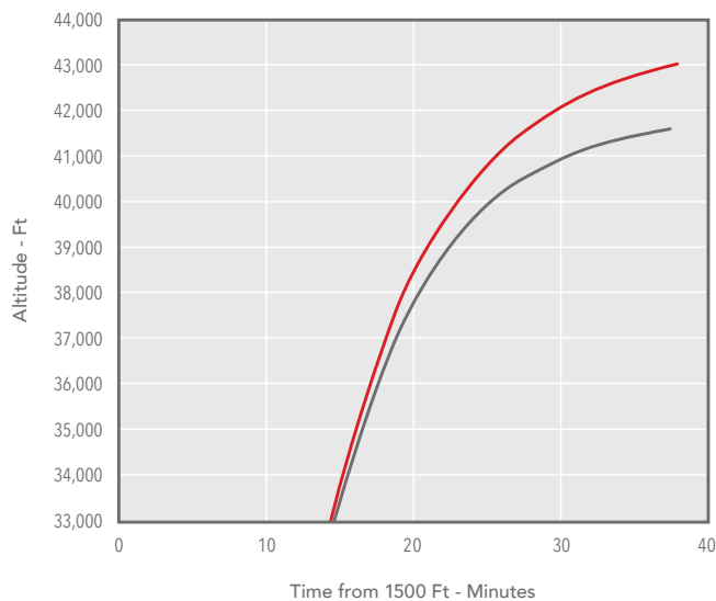
FALCON 50EX CLIMB TIME
