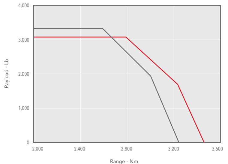
FALCON 50EX PAYLOAD RANGE
