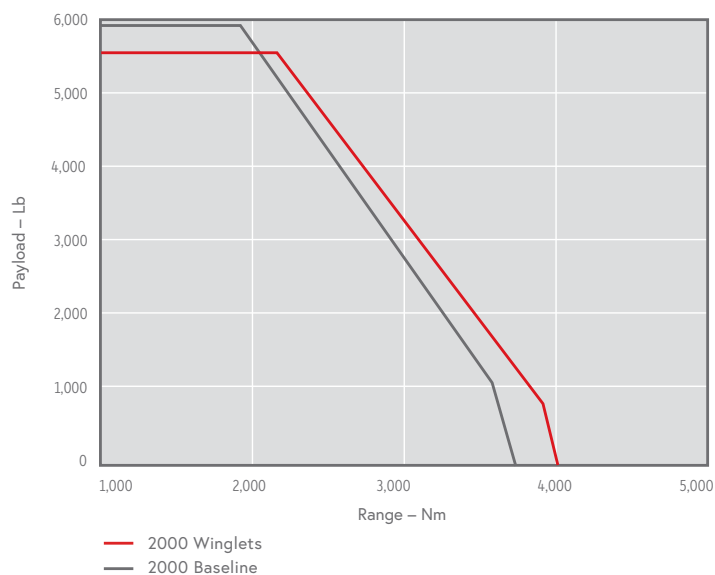
FALCON 2000 PAYLOAD RANGE
