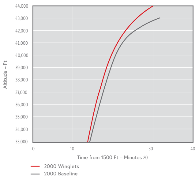
FALCON 2000 CLIMB TIME
