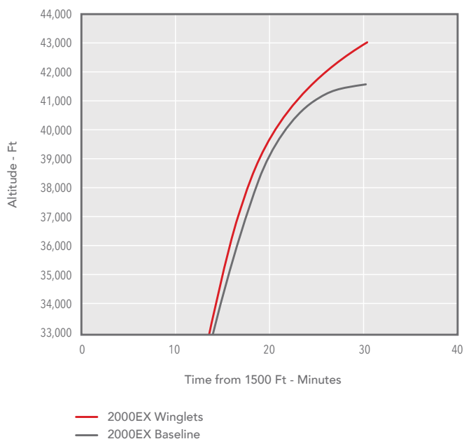
FALCON 2000EX CLIMB TIME
