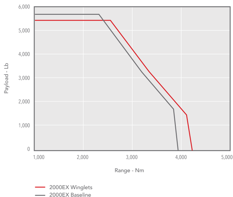
FALCON 2000EX PAYLOAD RANGE
