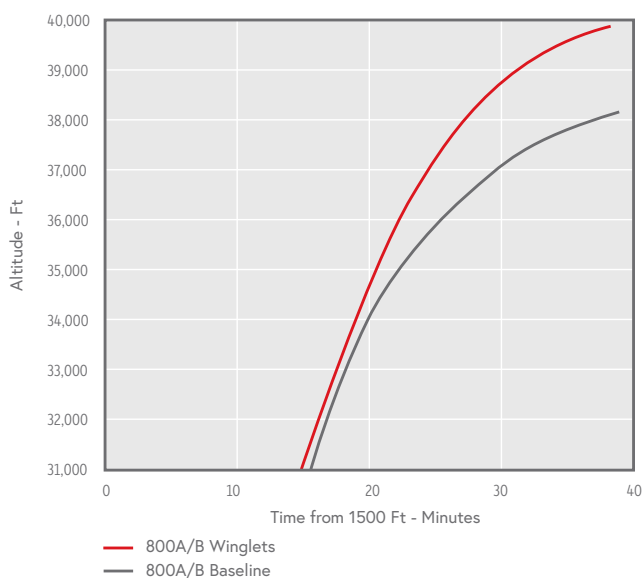
CLIMB TIME
