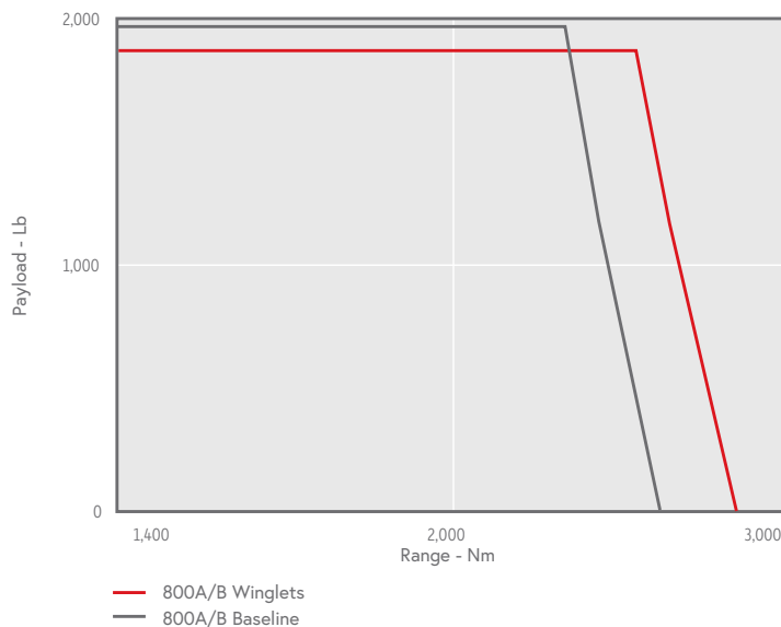
PAYLOAD RANGE
