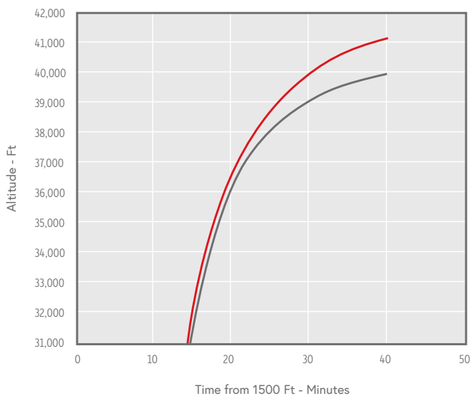
CLIMB TIME
