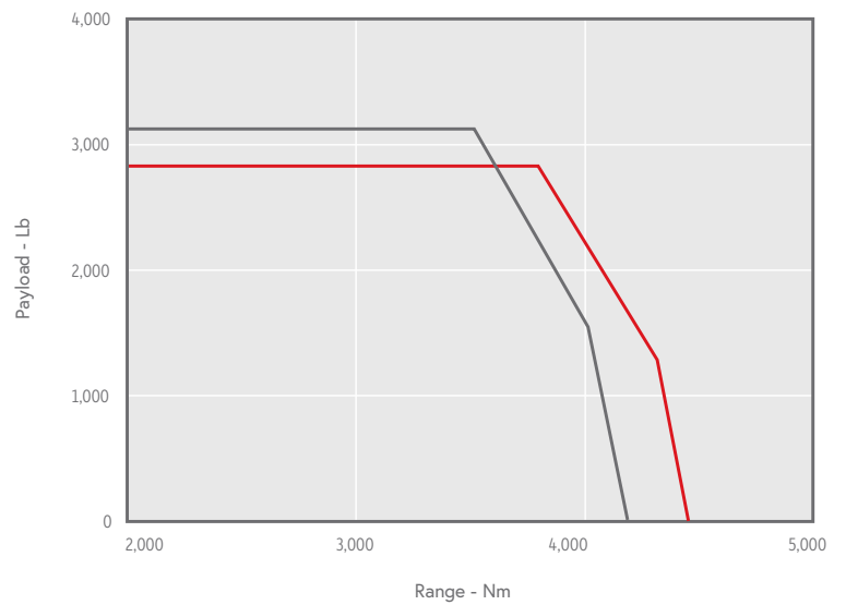
PAYLOAD RANGE
