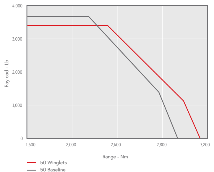
PAYLOAD RANGE
