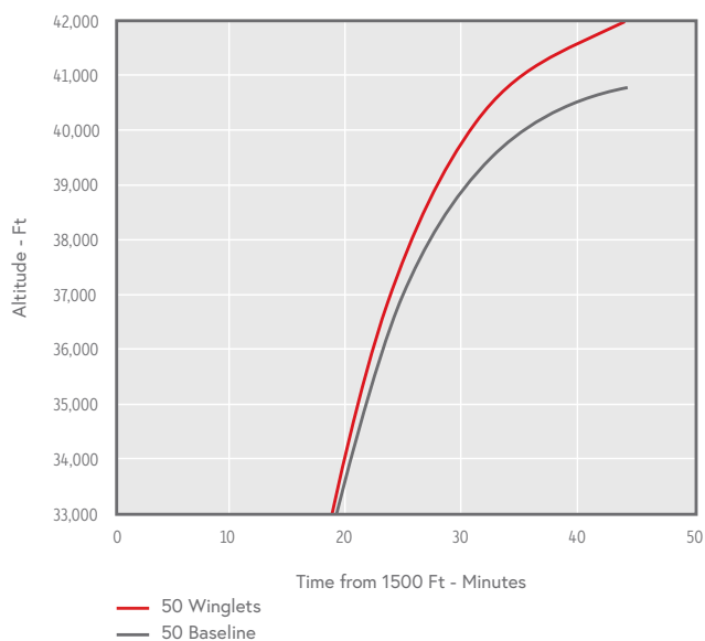
CLIMB TIME
