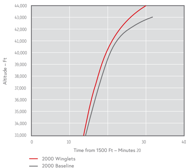
CLIMB TIME
