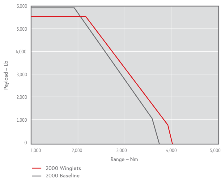
PAYLOAD RANGE
